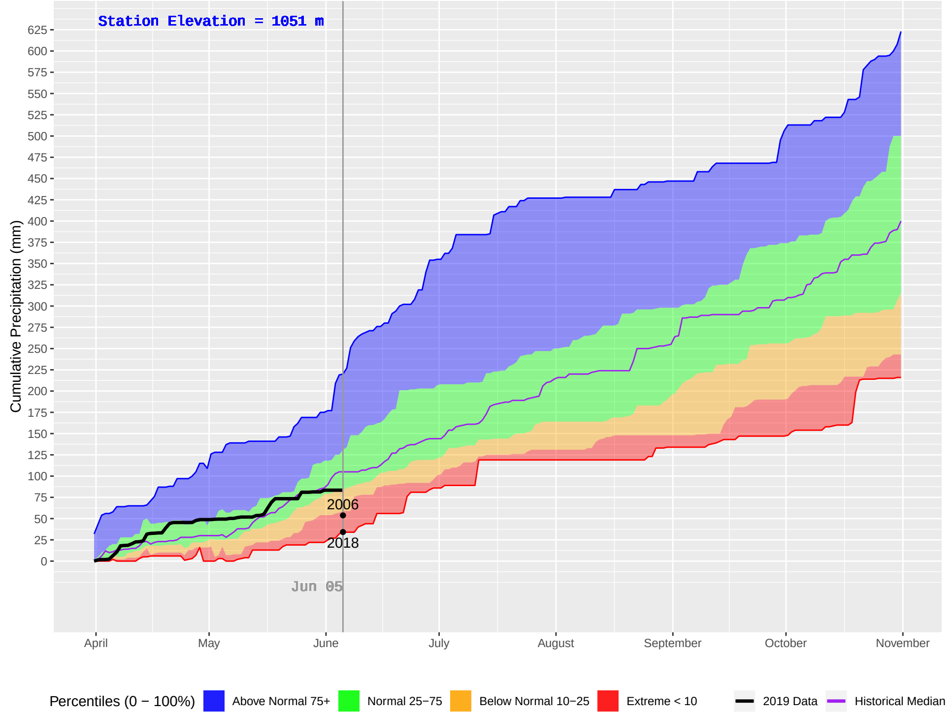
GOATHAVEN (886) : Historical (2005–2018), Current (2019) Daily Cumulative Precipitation
