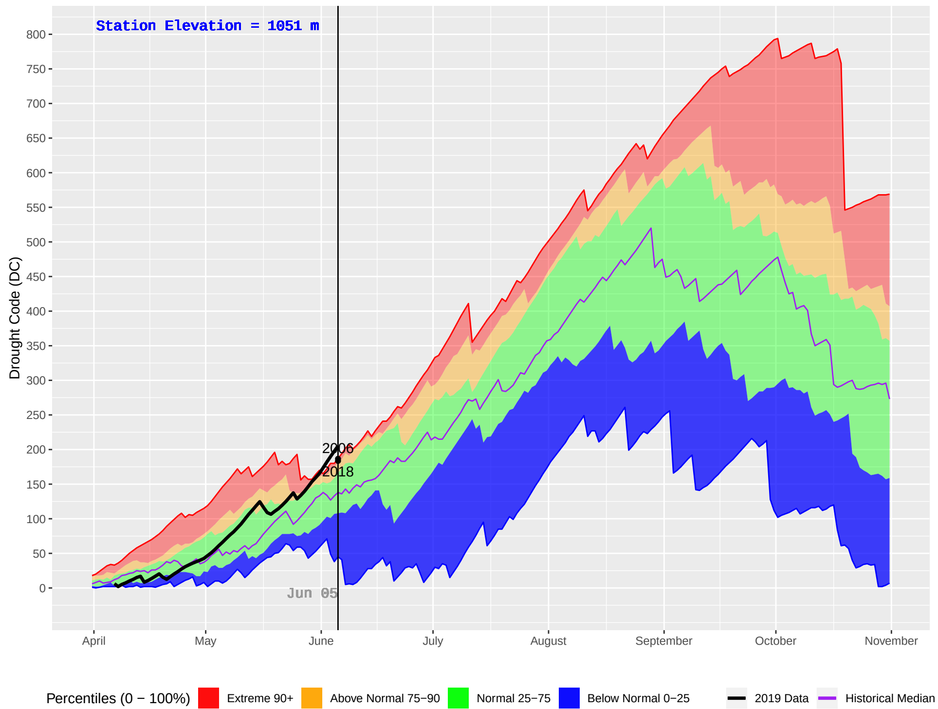
GOATHAVEN (886) : Historical (2005–2018) and Current (2019) Daily Drought Code (DC)
