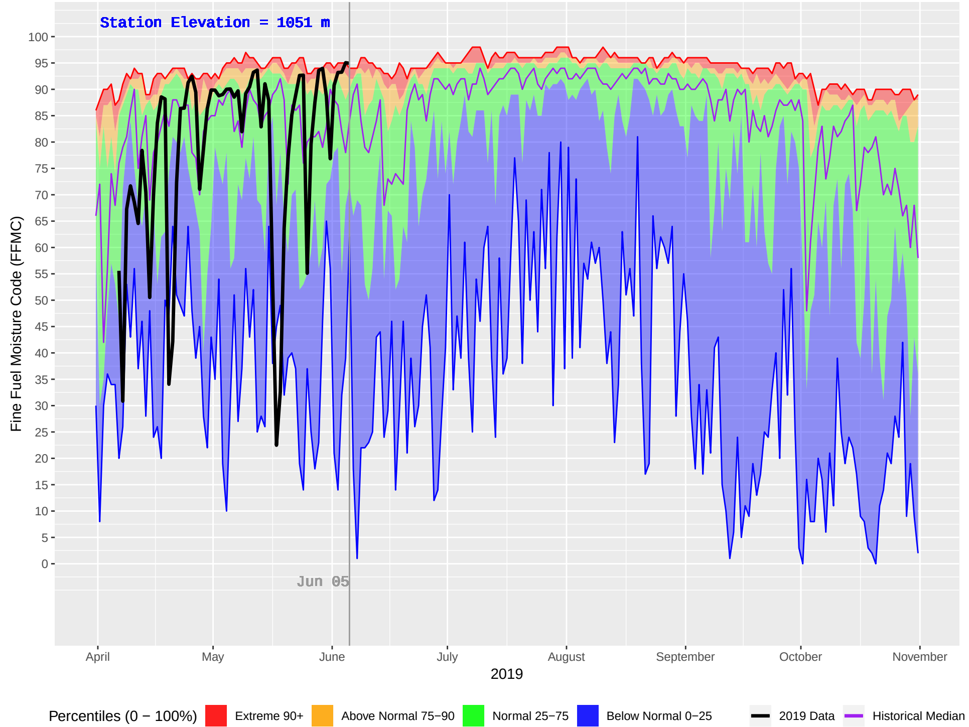
GOATHAVEN (886) : Historical (2005–2018) and Current (2019) Daily Fine Fuel Moisture Code (FFMC)
