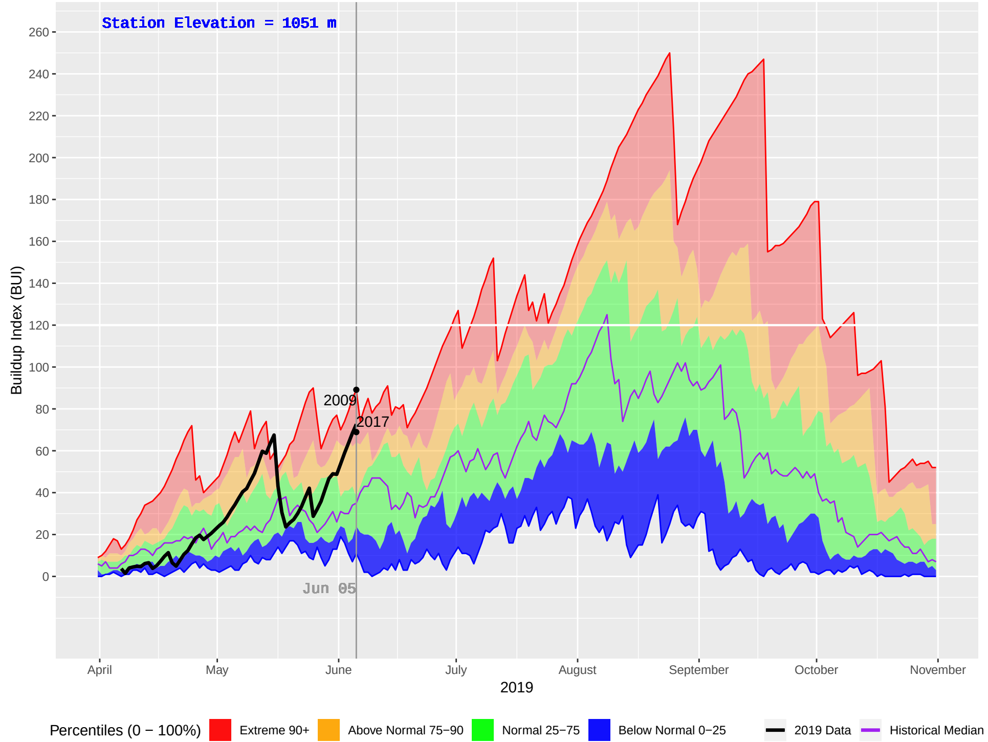
GOATHAVEN (886) : Historical (2005–2018), Current (2019) Daily Buildup Index (BUI)
