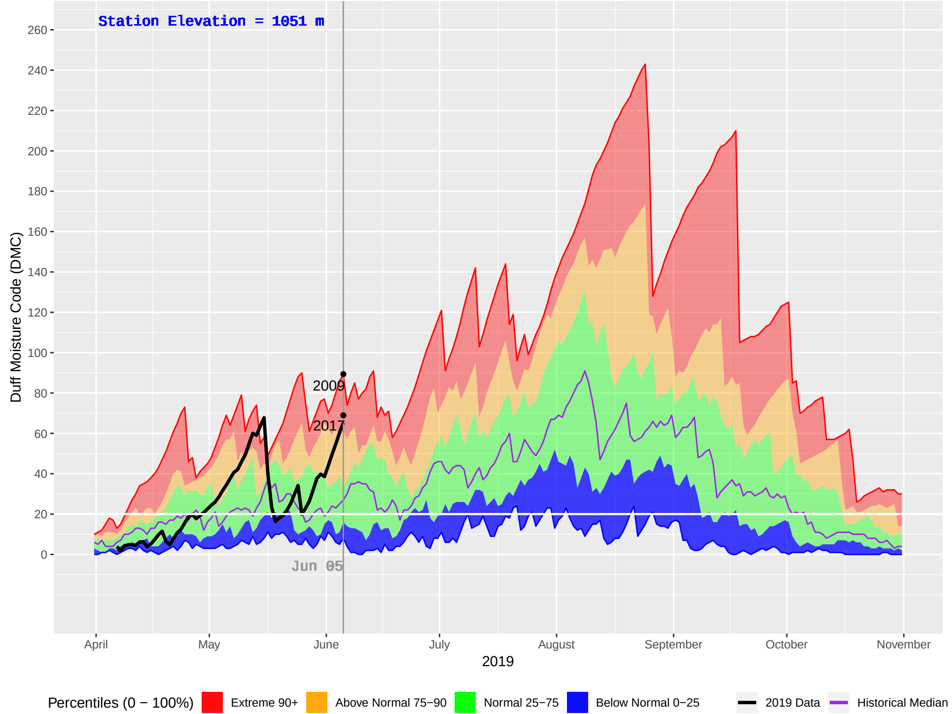
GOATHAVEN (886) : Historical (2005–2018), Current (2019) Daily Duff Moisture Code (DMC)
